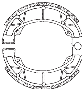
◀ cod. CP00219 Coppia ceppi \varnothing 110 x 25
