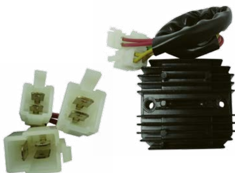
◀ cod. HN1022 Honda Applications 12 Volt Regulator Rectifier Assembly
