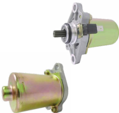
◀ cod. 19595N Chinese PMDD 12 Volt, CCW, 11-Tooth Pinion
