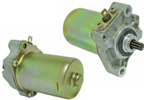
◀ cod. 37044N China (Made) PMDD 12 Volt, CCW, 9-Tooth Pinion
