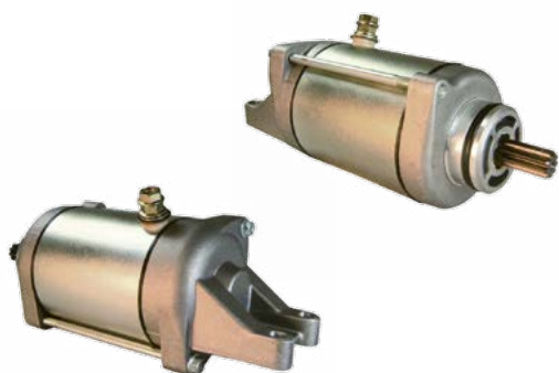
◀ cod. 18733N Mitsuba PMDD 12 Volt, CCW, 9-Tooth Spline
