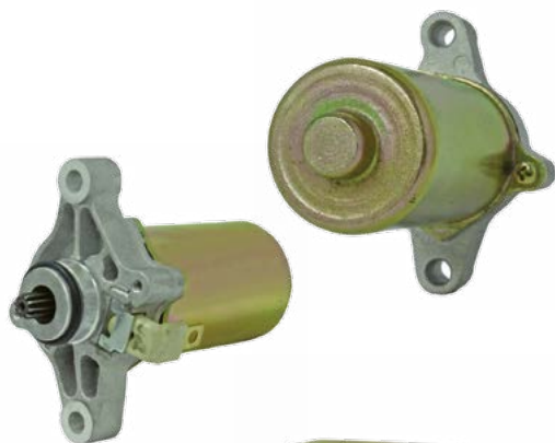
◀ cod. 37010N China (Made) PMDD 12 Volt, CCW
