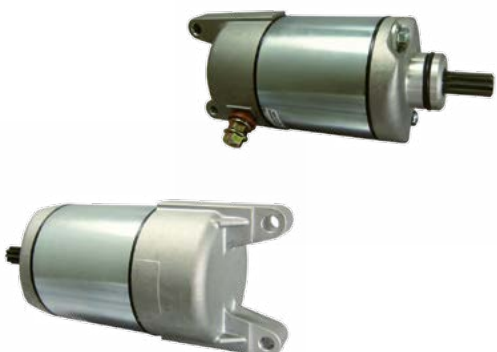
◀ cod. 18702N Mitsuba PMDD 12 Volt, CCW, 9-Tooth Spline
