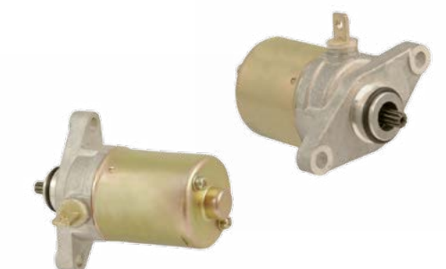
◀ cod. 19587N China (Made) PMDD 12 Volt, CCW, 9-Tooth Pinion
