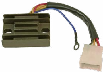
◀ cod. PL1011N Aprilia Motorcycles 12 Volt Regulator Rectifier Assembly
