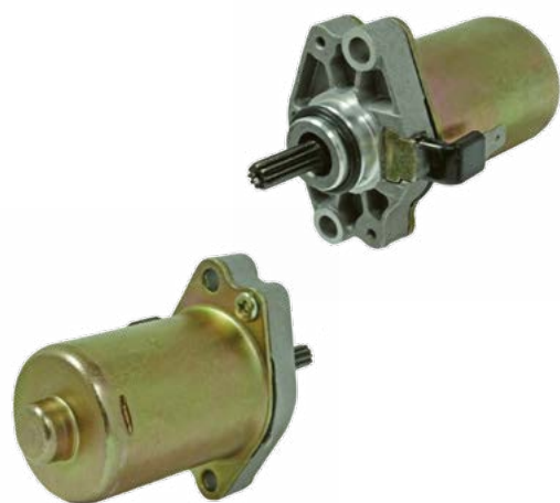
◀ cod. 37036N China (Made) PMDD 12 Volt, CCW, 10-Tooth Pinion
